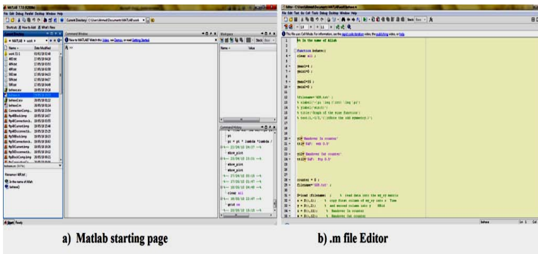
Figure 3.10 Visualization software
