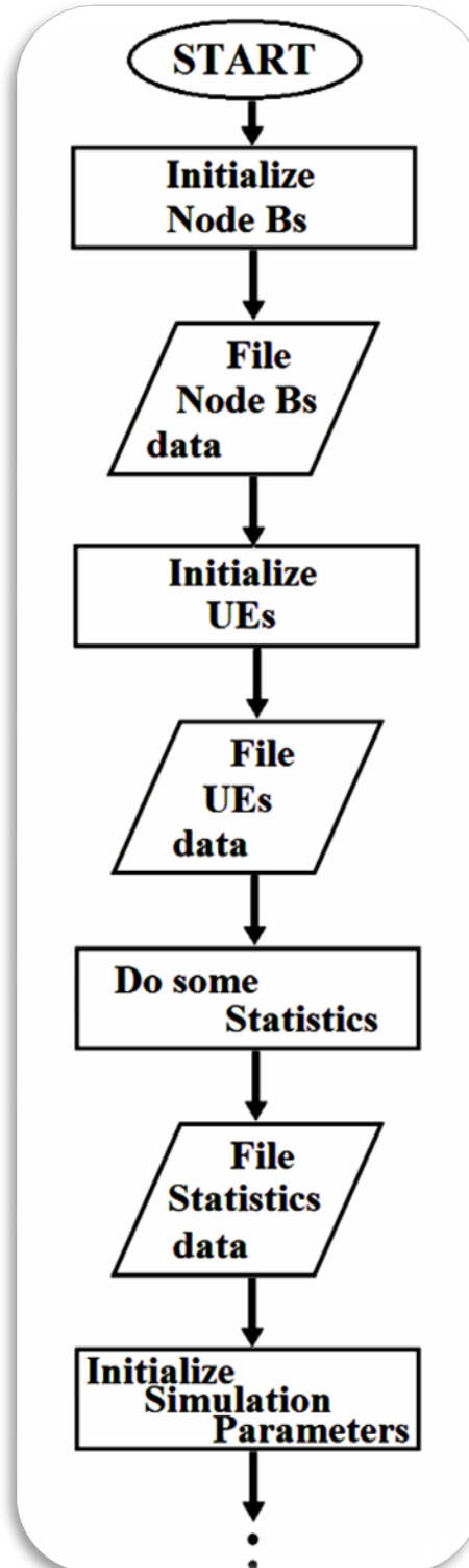
Figure 3.2 Initialization phase
