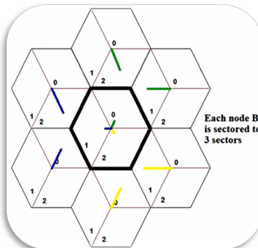
Figure 3.7 Performed sectoring
